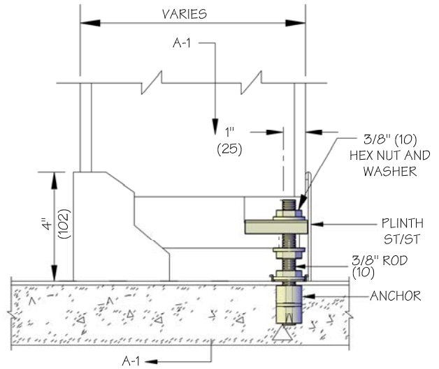
DETAIL A
